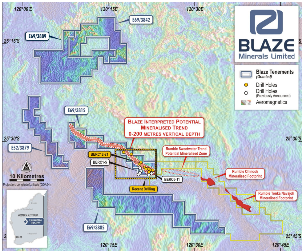
Figure 3: Blaze Regional Drillhole Location on Aeromagnetics
