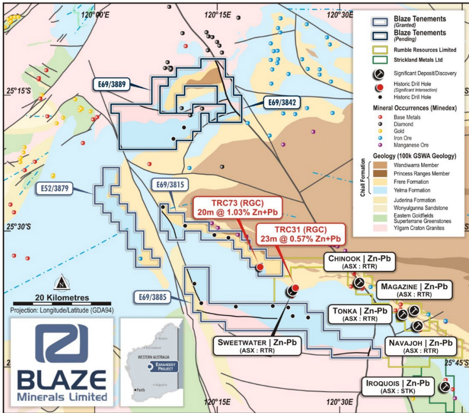
Figure 2: Location of Earaheedy Basin Tenure
